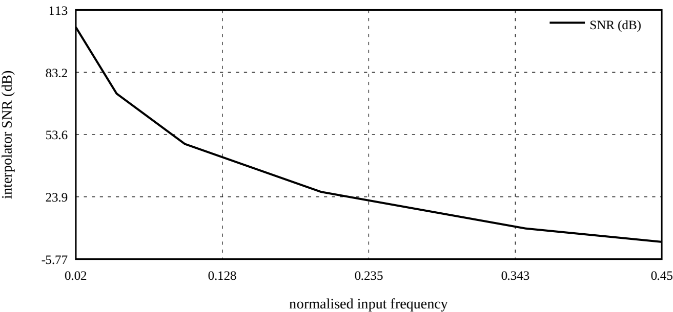
Figure 40. Cubic Farrow interpolation accuracy. Choosing the oversampling ratio is choosing a point on this curve.
