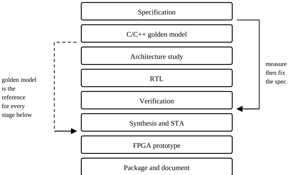
Figure 43. The solo flow. The dashed line is the one that matters: the golden model is the reference for every stage below it, which is what replaces organisational independence.
