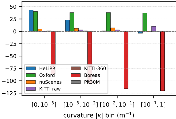
H2 falsified across 7 datasets at 10 Hz
