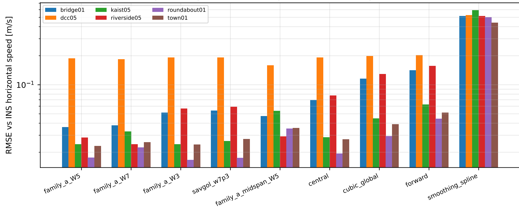
HeLiPR Layer 3: alignment with independent INS velocity (lower is better)
