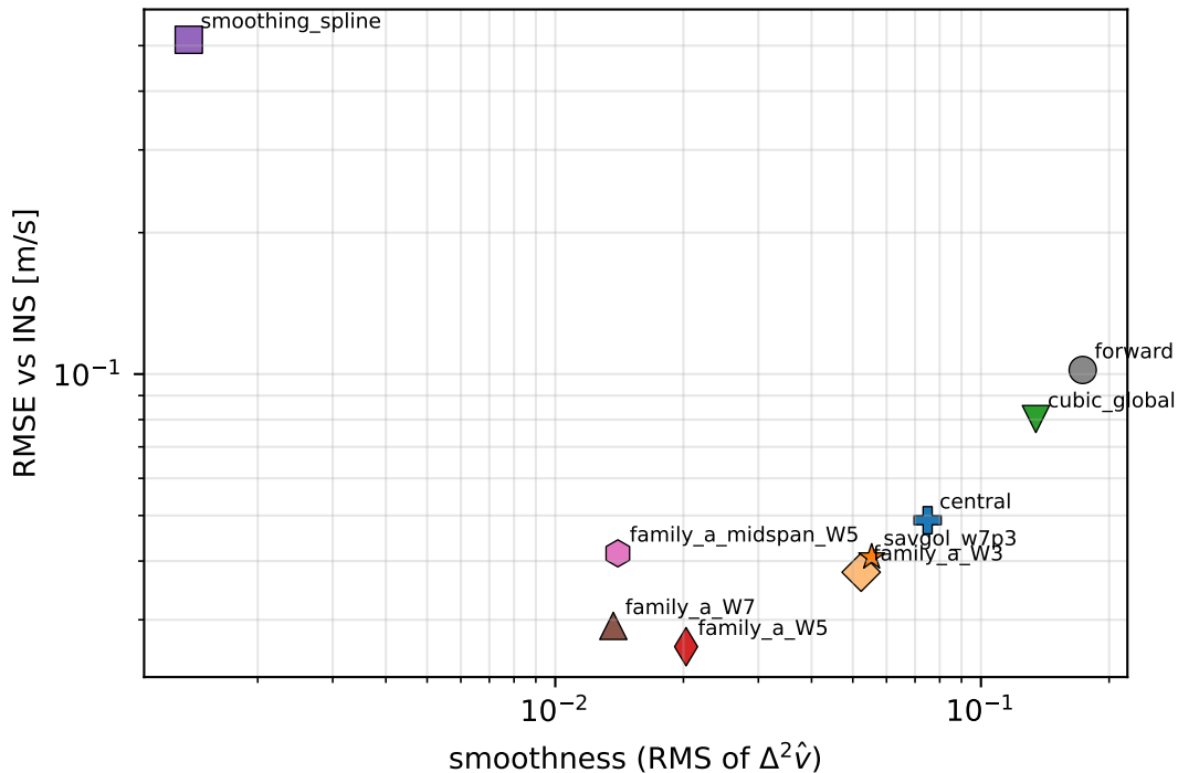
HeLiPR: smoothness vs INS-alignment (bottom-left = better)
