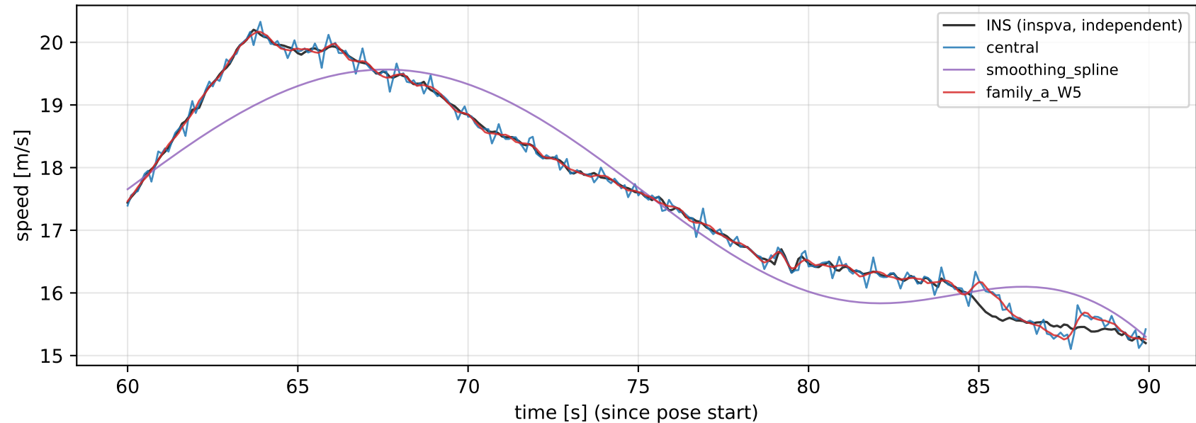
HeLiPR bridge01: pose-derived speed vs INS reference (window 60s..+30s)
