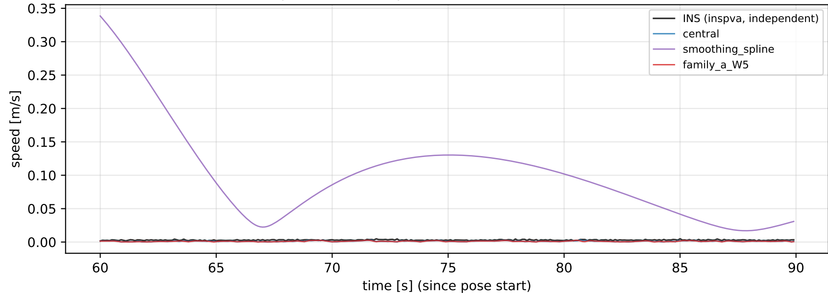
HeLiPR dcc05: pose-derived speed vs INS reference (window 60s..+30s)
