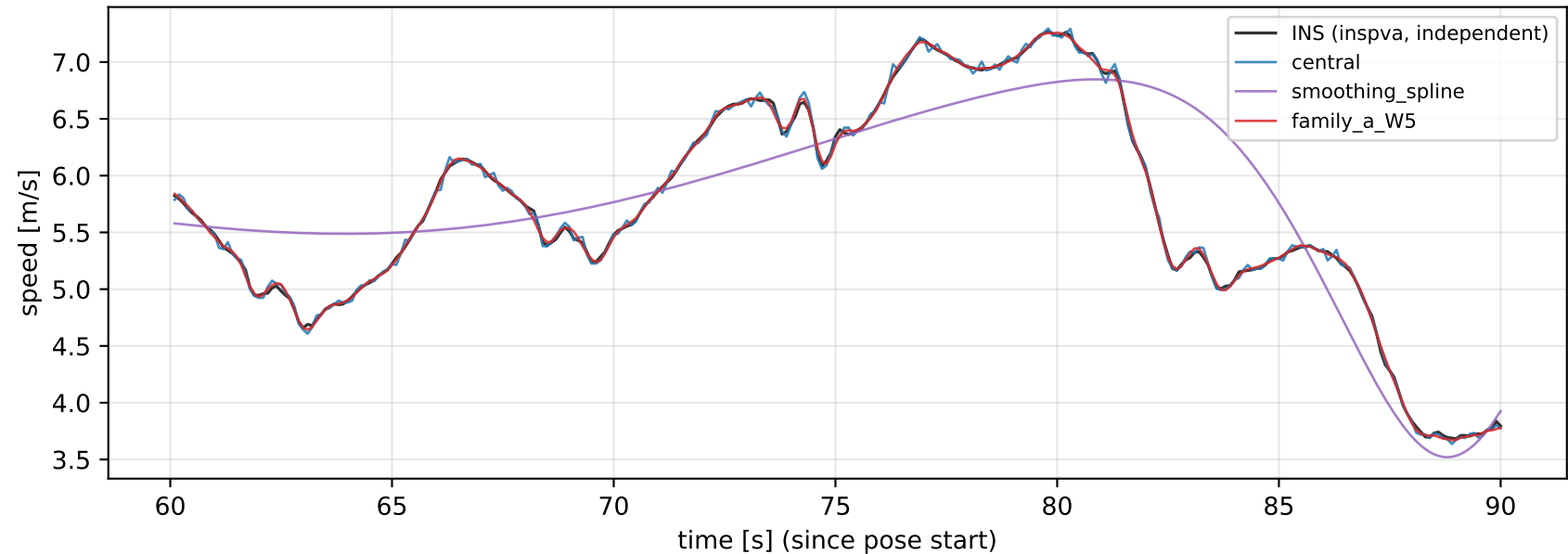
HeLiPR kaist05: pose-derived speed vs INS reference (window 60s..+30s)
