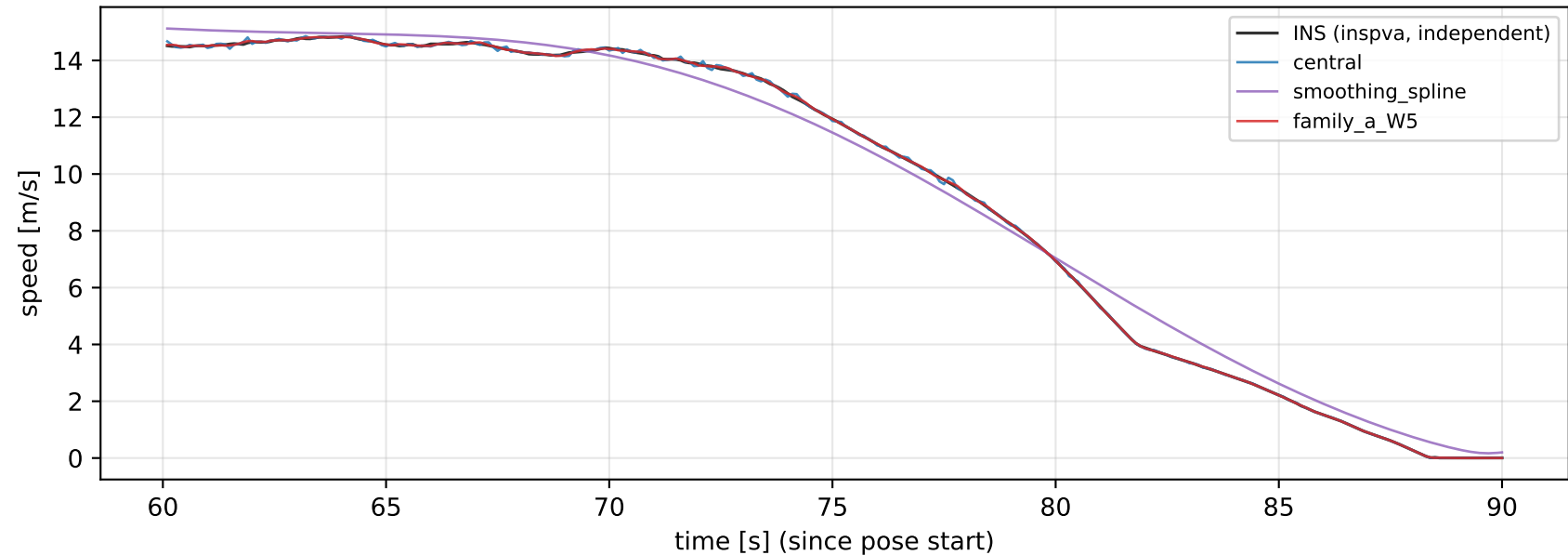
HeLiPR riverside05: pose-derived speed vs INS reference (window 60s..+30s)
