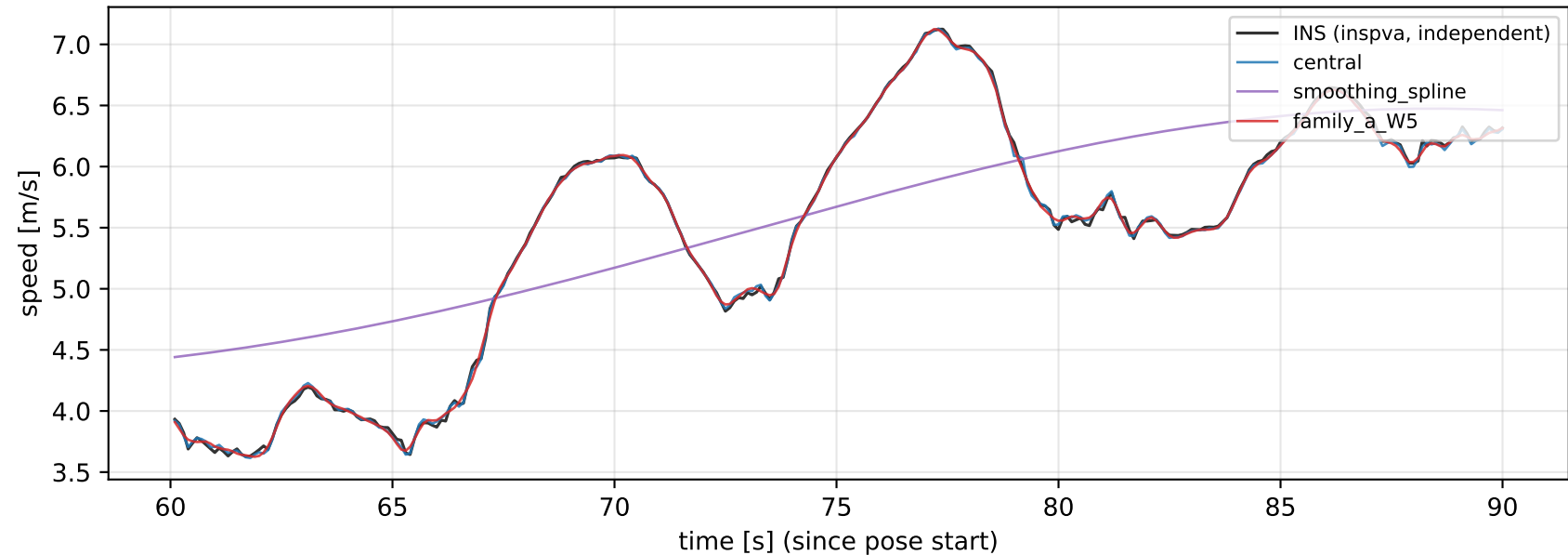
HeLiPR town01: pose-derived speed vs INS reference (window 60s..+30s)
