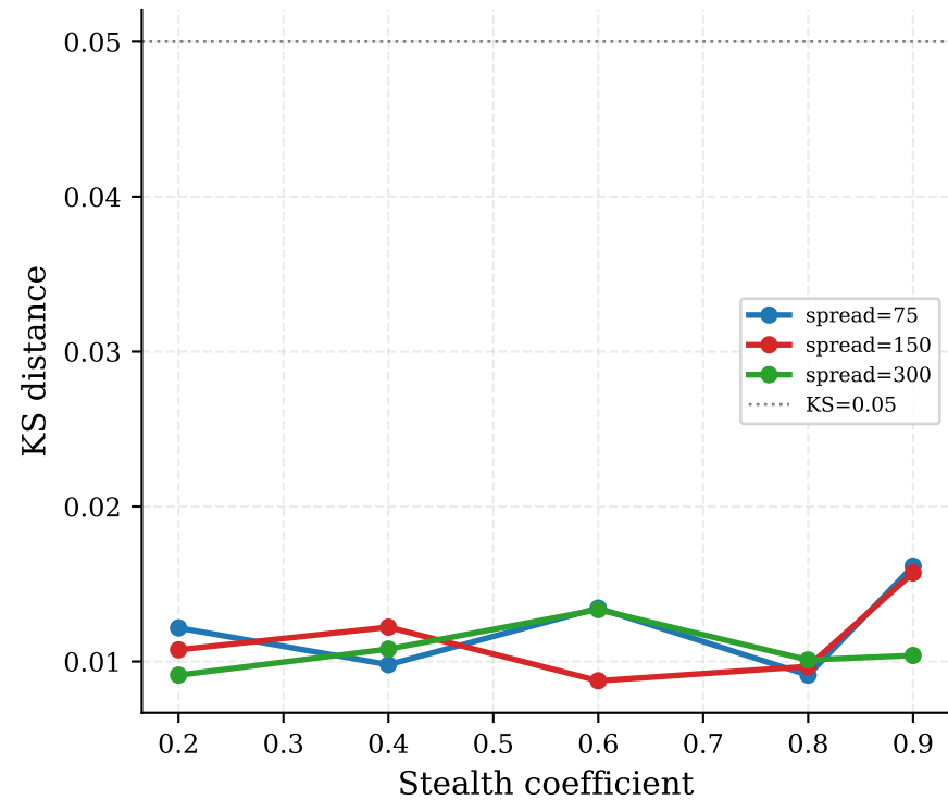
Stealthy: KS vs. Stealth (marginal exactly preserved)
