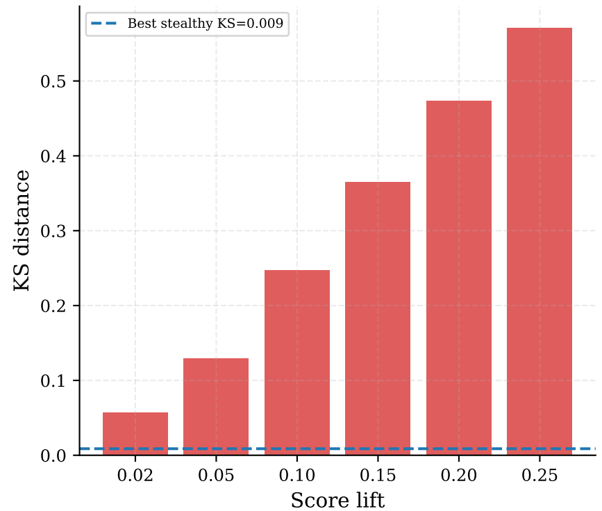
Naive: KS vs. Score Lift (marginal visibly shifted)
