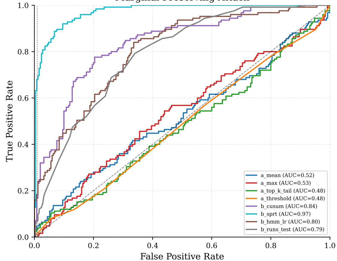
Marginal-Preserving Attack
