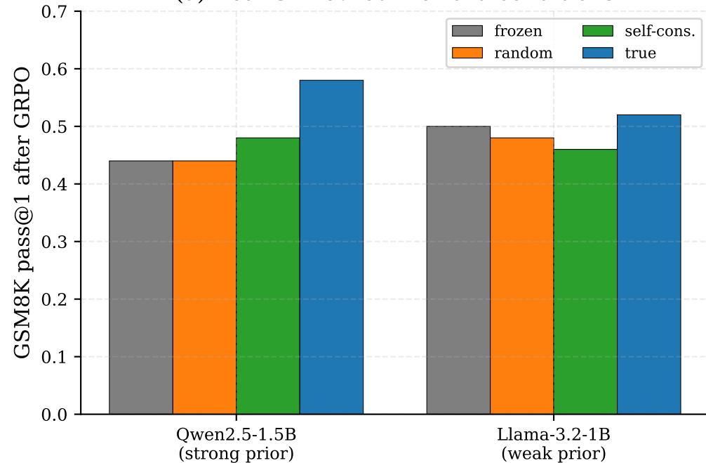
(a) Real GRPO: four reward conditions
