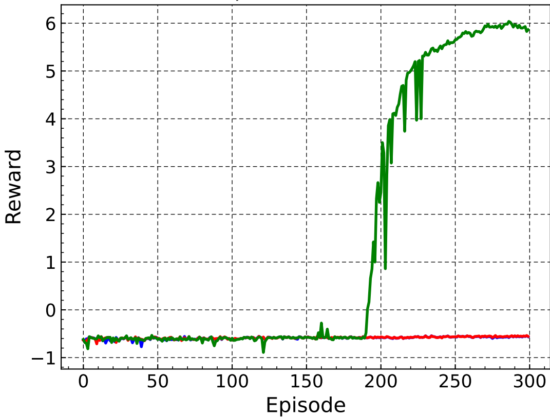
Episode Rewards
