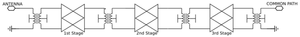
Figure 3.1: Proposed three-stage transformer-based bidirectional front-end architecture.
