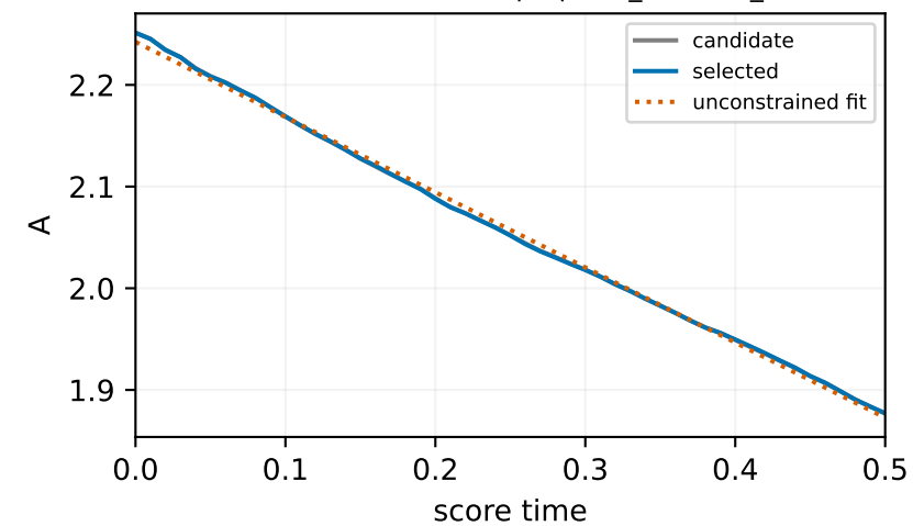
ck2:A:VAL116::NOS::proposal_spread
