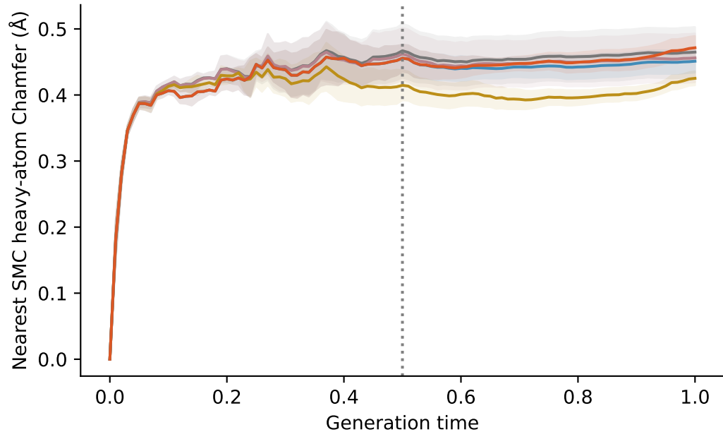
Distance to same-batch SMC samples (lower is closer; mean \pm batch SEM)
