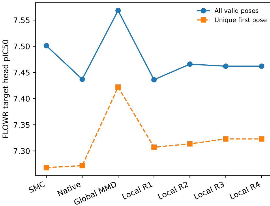
Prediction, not measured binding
