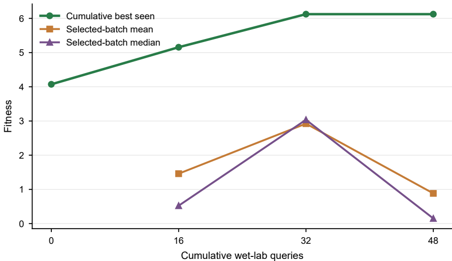
kg_3features_base, fold 2
