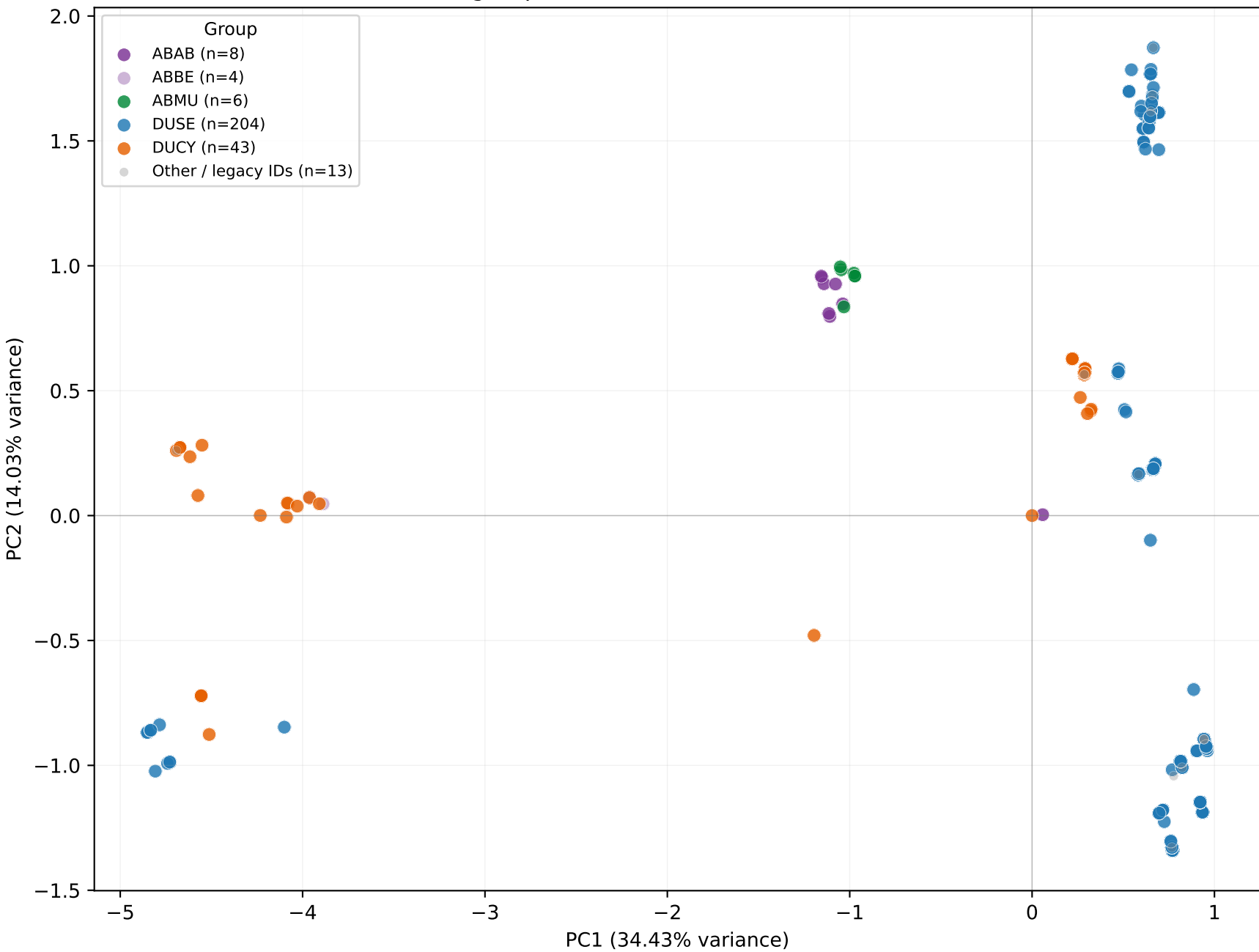
mtDNA PCA grouped as DUSE / DUCY / ABAB / ABBE / ABMU
