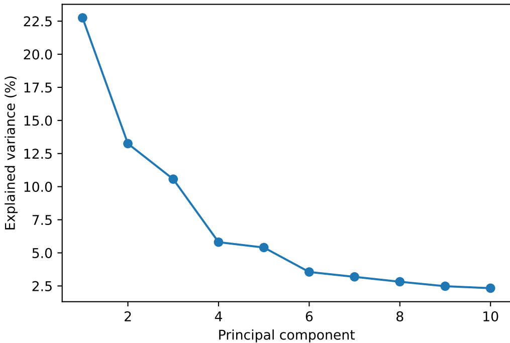
Mitochondria PCA scree (presentation replacement)
