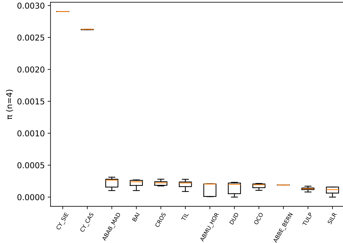
Sample-size-standardized chloroplast \pi
