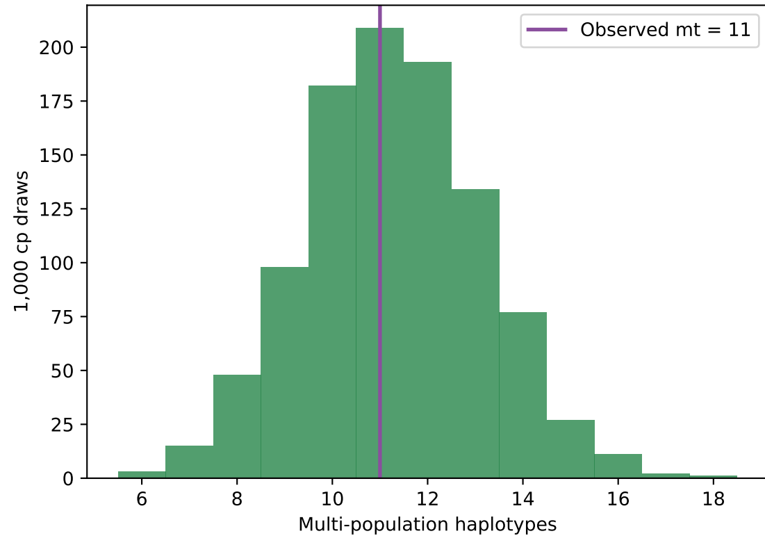
146-site marker-count sensitivity
