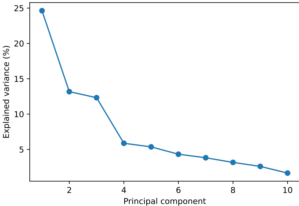
Chloroplast PCA scree (presentation replacement)
