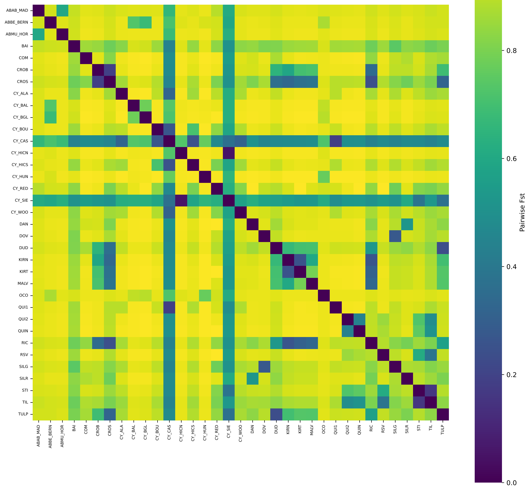
cpDNA pairwise Fst among populations
