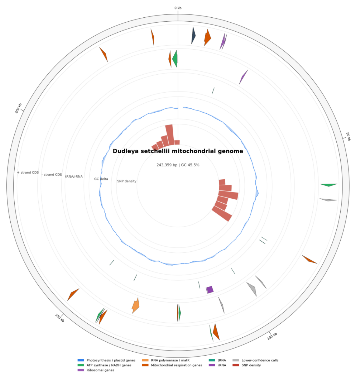
B. mtDNA circular genome map
