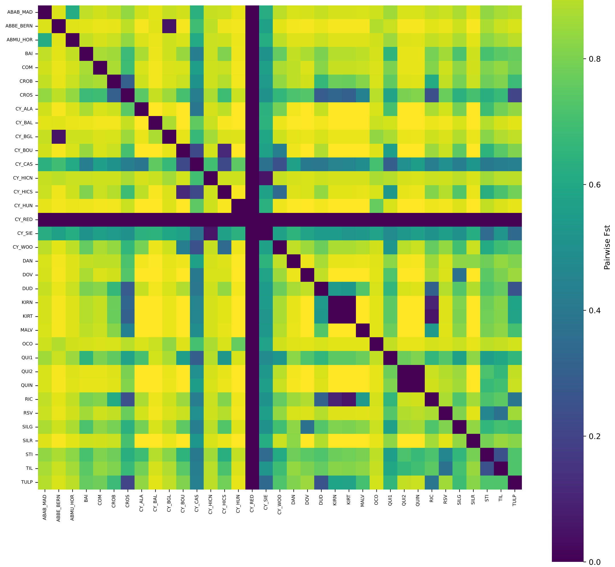
mtDNA pairwise F_{st} among populations
