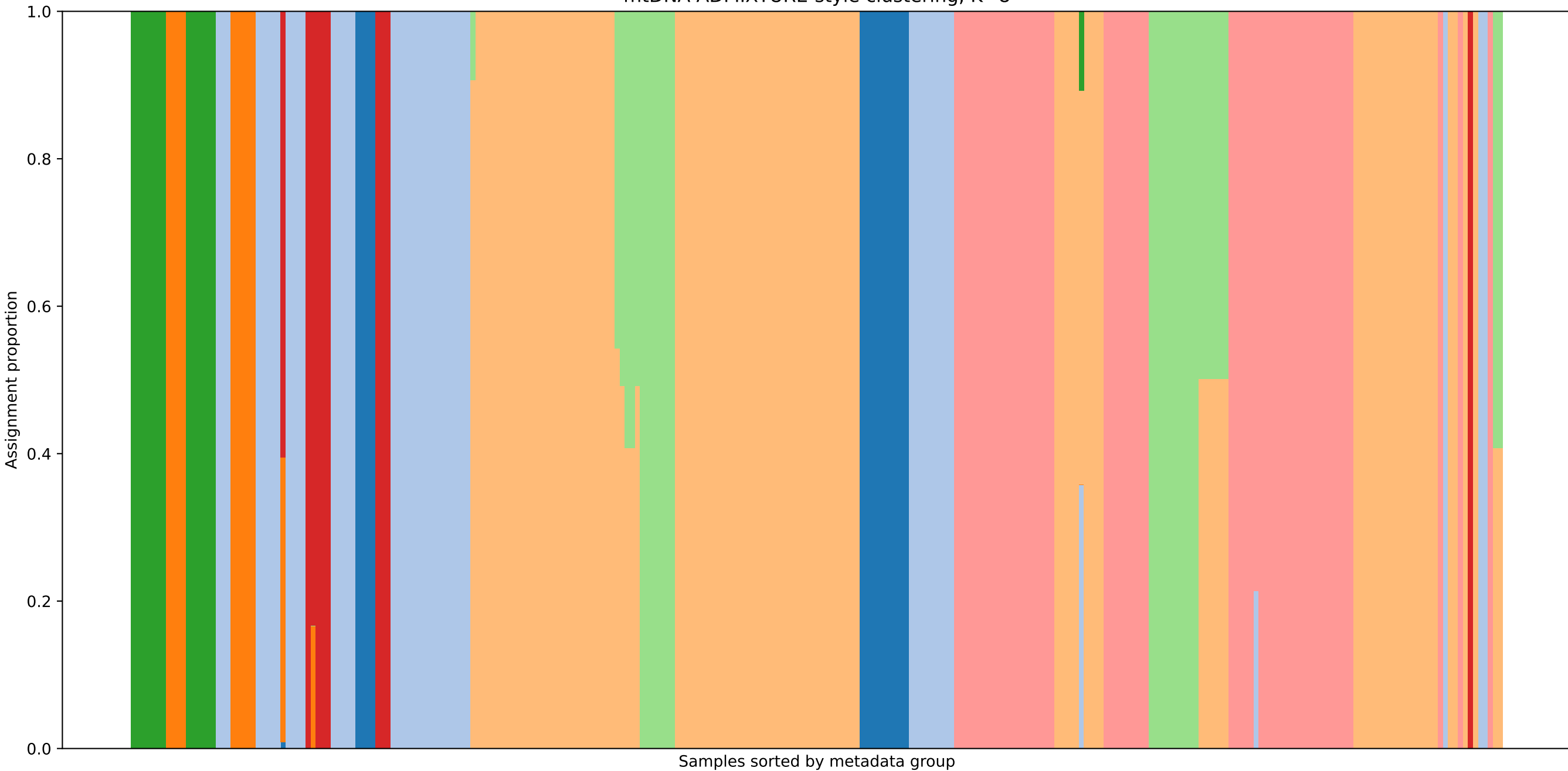
mtDNA ADMIXTURE-style clustering, K=8
