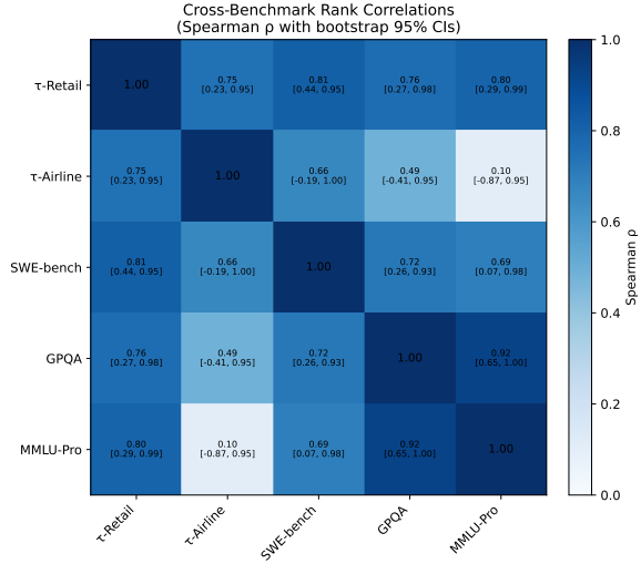
Figure 1: Spearman rank correlations between benchmarks (pairwise complete, n = 6 –15 per pair), with percentile bootstrap 95% CIs (10,000 resamples) shown under each off-diagonal estimate. Correlations between \tau -Airline and the reasoning benchmarks are non-significant ( p > 0.05 ), and their CIs are wide enough to include zero. The block structure suggests at least two latent factors: a “tool-use” cluster ( \tau -Retail, \tau -Airline, SWE-bench) and a “reasoning” cluster (GPQA, MMLU-Pro), with \tau -Airline carrying most of the discriminant signal.
