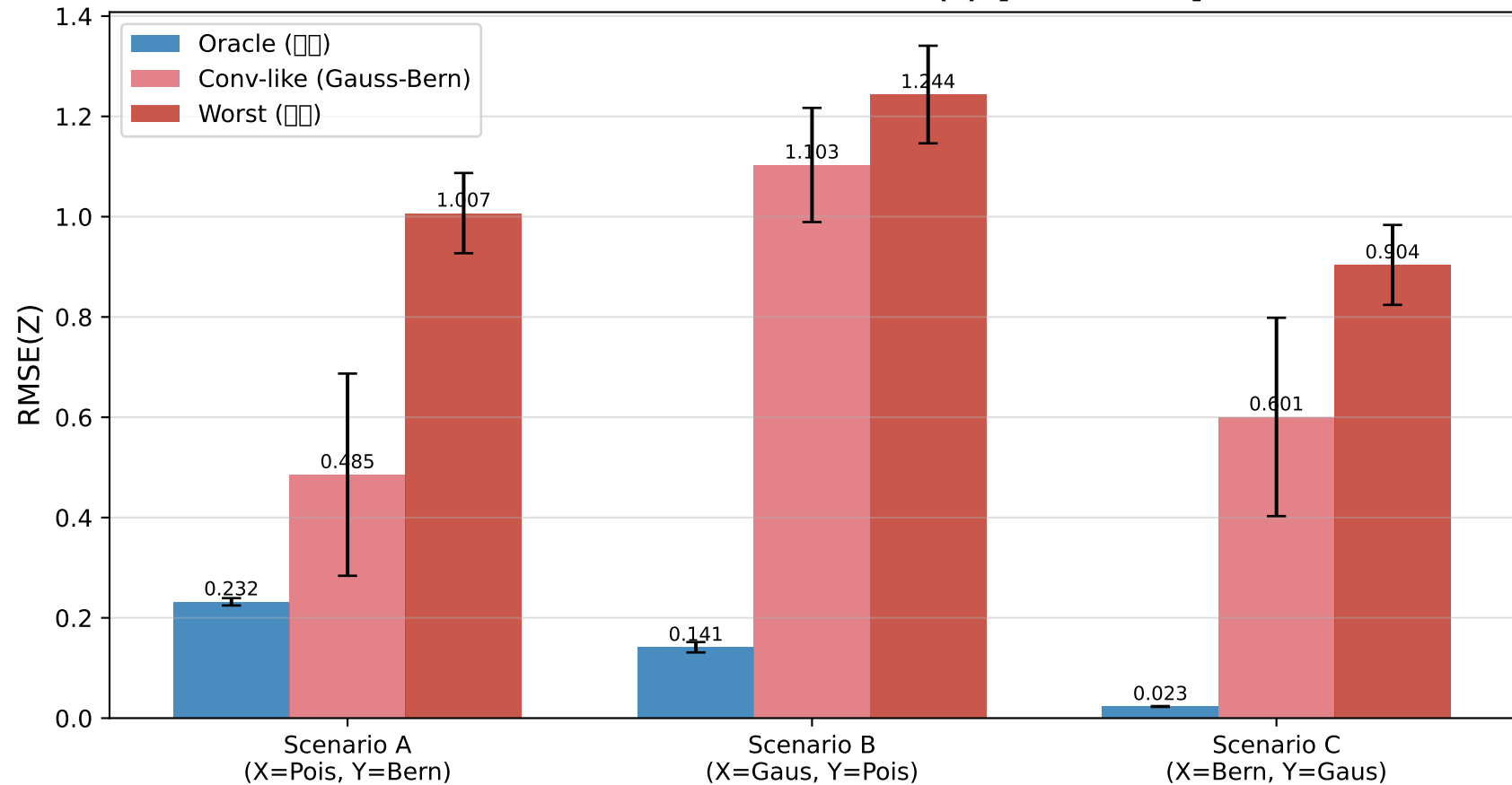
Oracle vs Conv-like vs Worst RMSE(Z) [Fixed model]
