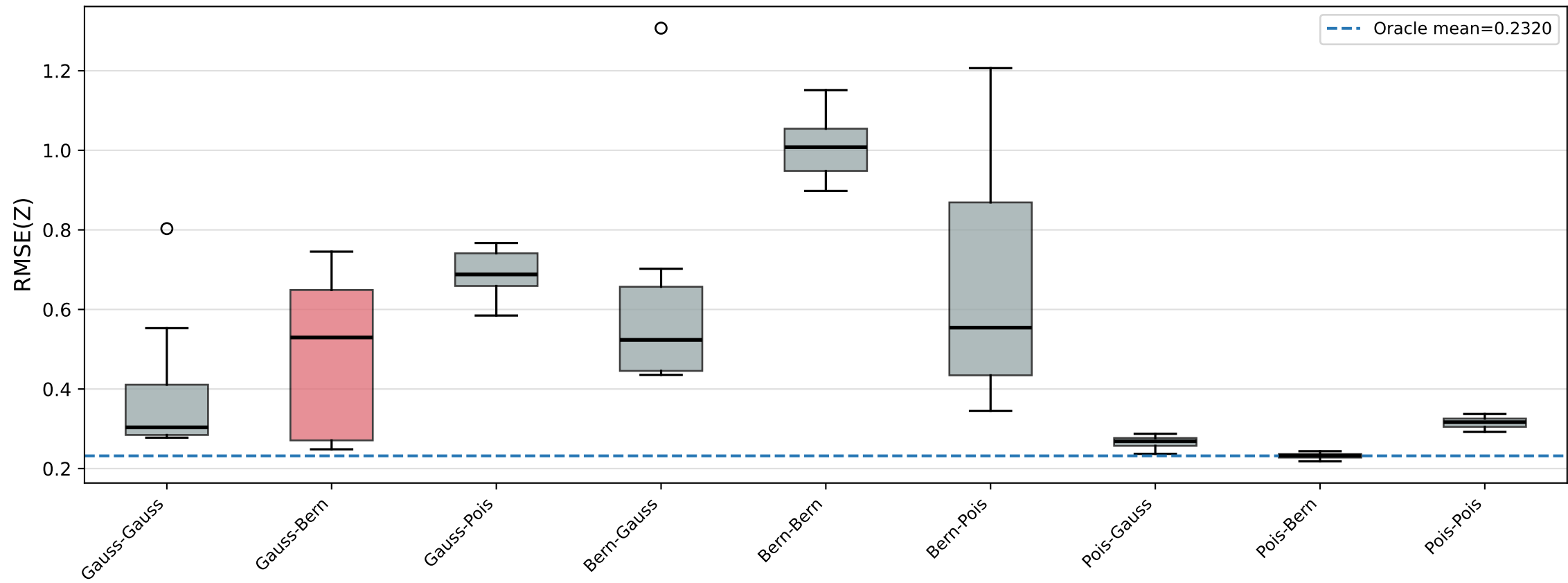
Scenario A RMSE(Z) distribution [Fixed model] True: X=Poisson, Y=Bernoulli (Oracle=blue, Conv-like=red, 10 trials)
