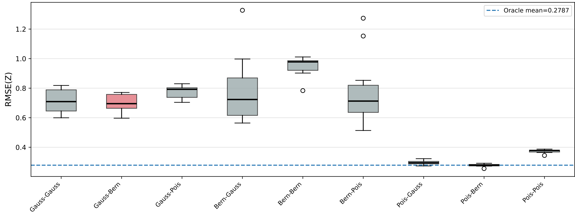
Scenario A RMSE(Z) distribution [Old model, 0.5 ] True: X=Poisson, Y=Bernoulli (Blue=Oracle, Red=Conv-like, 10 trials)
