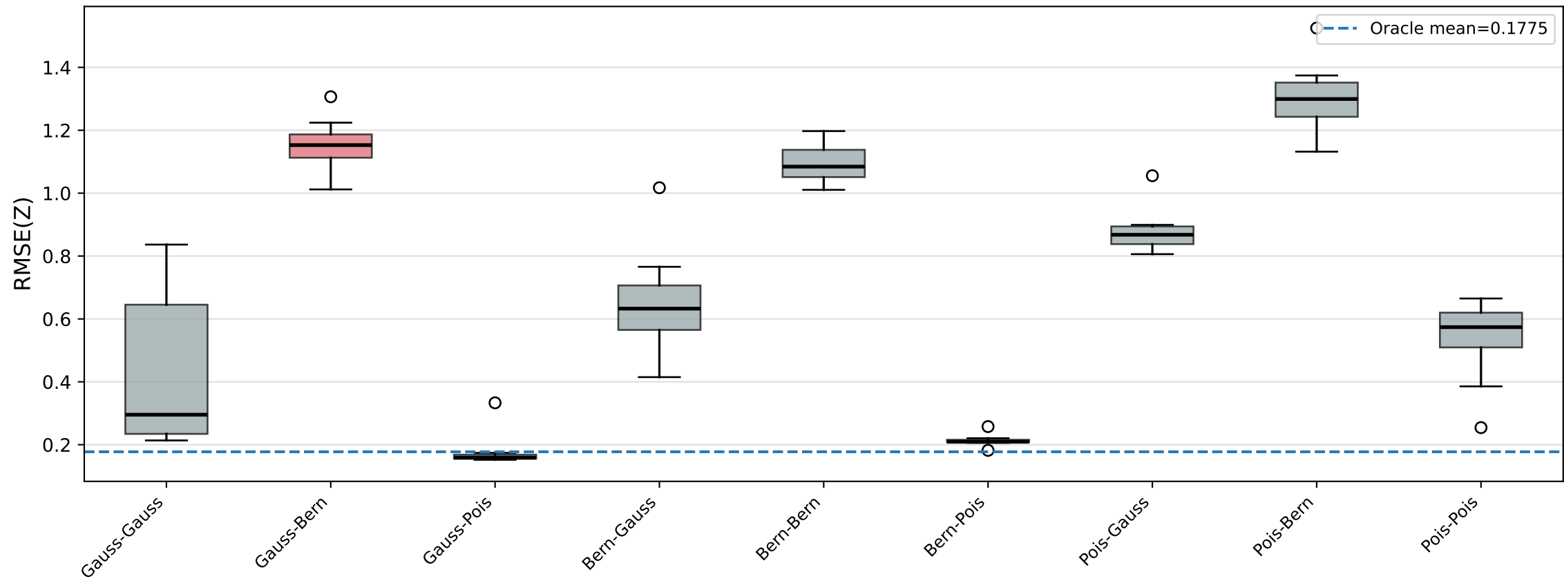
Scenario B RMSE(Z) distribution [Old model, 0.5 ] True: X=Gaussian, Y=Poisson (Blue=Oracle, Red=Conv-like, 10 trials)
