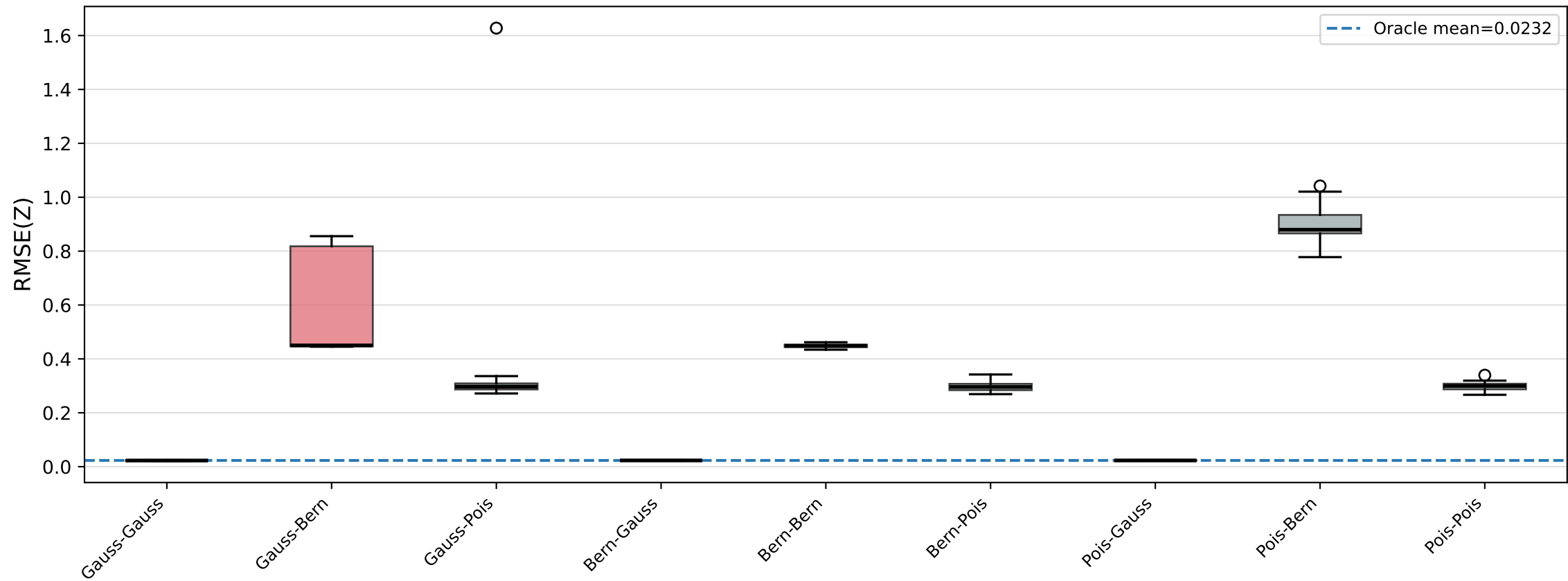
Scenario C RMSE(Z) distribution [Fixed model] True: X=Bernoulli, Y=Gaussian (Oracle=blue, Conv-like=red, 10 trials)
