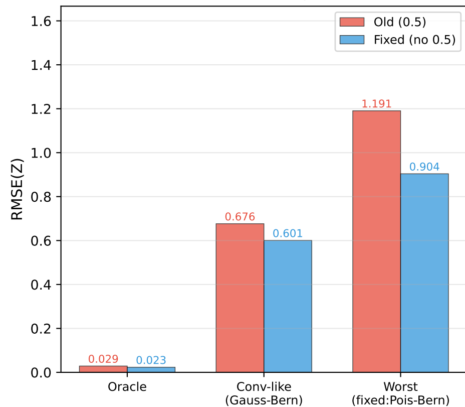
Scenario C: X=Bern, Y=Gaus
