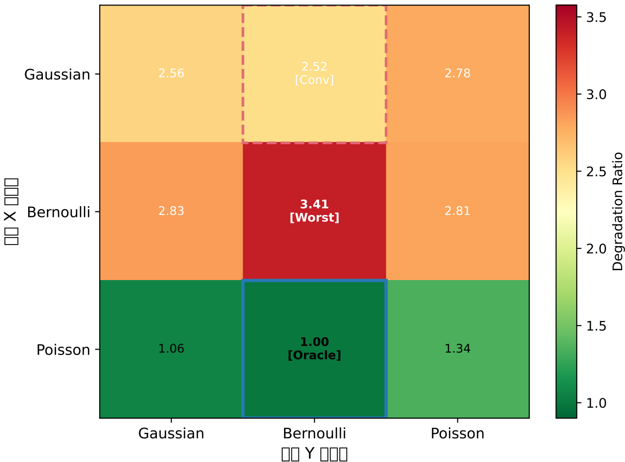
Scenario A Degradation Ratio [Old model: 0.5] True: X=Poisson, Y=Bernoulli (n=150, d=15, k=3, 10 trials)
