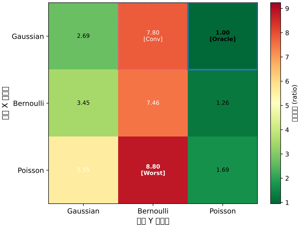
Scenario B \frac{\text{Oracle}}{\text{Conv}} \text{ (ratio)} [Fixed model] True: X=Gaussian, Y=Poisson (n=150, d=15, k=3, 10 trials)
