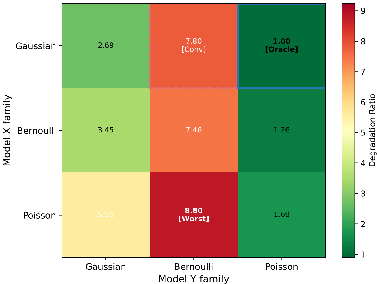
Scenario B Degradation Ratio [Fixed model: no 0.5] True: X=Gaussian, Y=Poisson (n=150, d=15, k=3, 10 trials)
