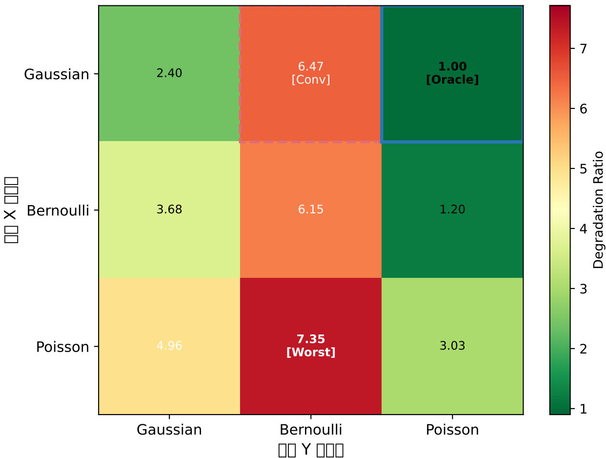
Scenario B Degradation Ratio [Old model: 0.5 ] True: X=Gaussian, Y=Poisson (n=150, d=15, k=3, 10 trials)
