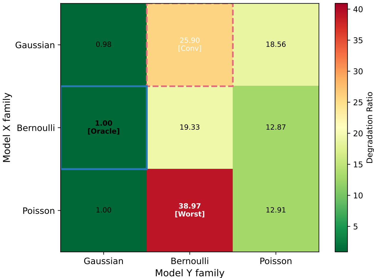
Scenario C Degradation Ratio [Fixed model: no 0.5] True: X=Bernoulli, Y=Gaussian (n=150, d=15, k=3, 10 trials)
