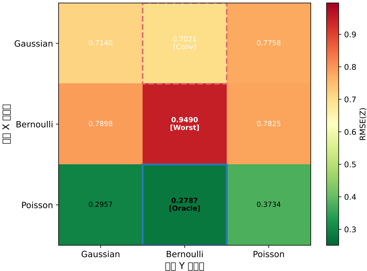
Scenario A RMSE(Z) [Old model: 0.5 \square\square ] True: X=Poisson, Y=Bernoulli (n=150, d=15, k=3, 10 trials)
