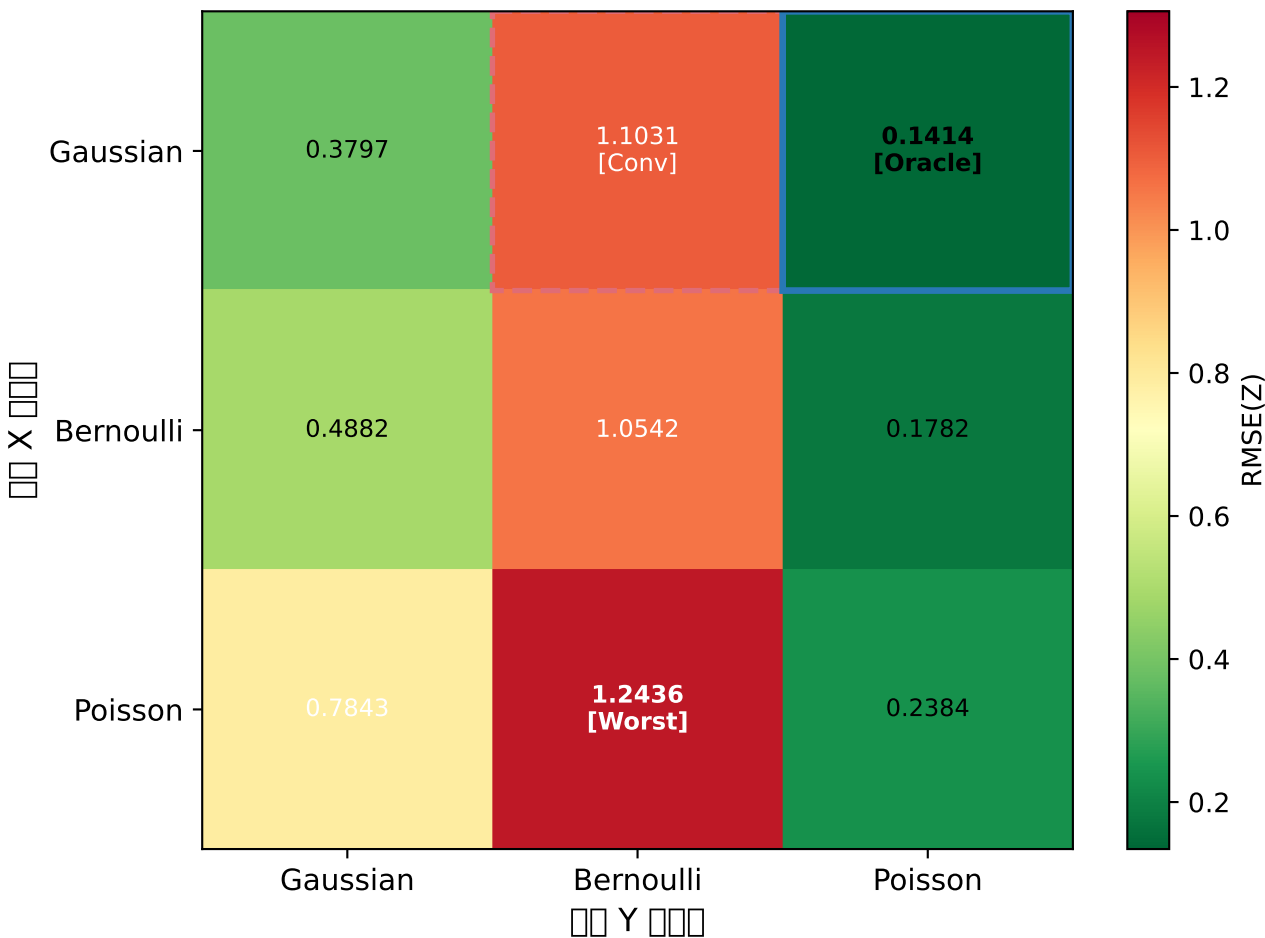
Scenario B RMSE(Z) [Fixed model] True: X=Gaussian, Y=Poisson (n=150, d=15, k=3, 10 trials)
