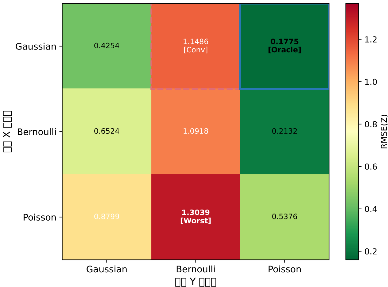
Scenario B RMSE(Z) [Old model: 0.5 \square\square ] True: X=Gaussian, Y=Poisson (n=150, d=15, k=3, 10 trials)
