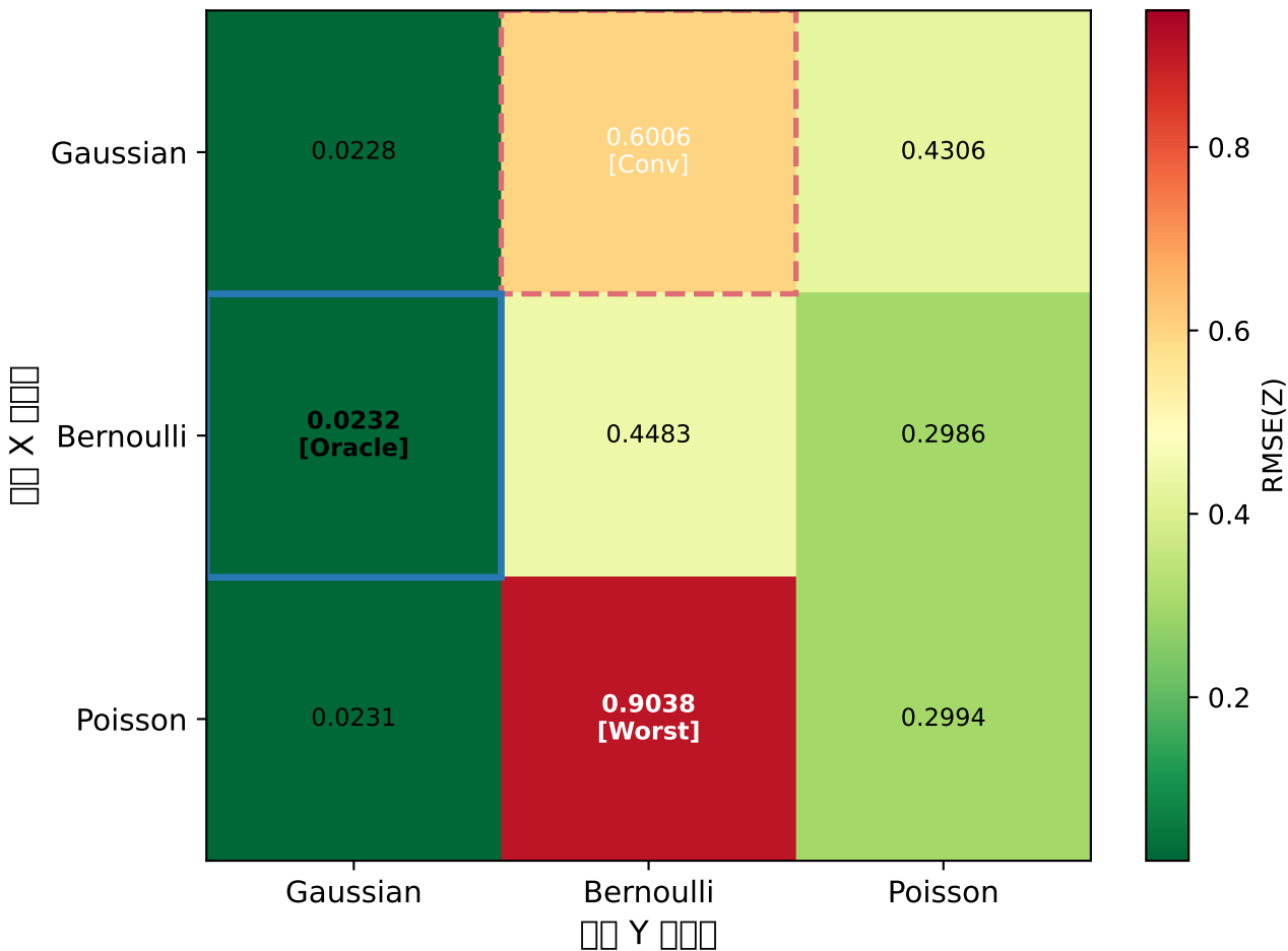
Scenario C RMSE(Z) [Fixed model] True: X=Bernoulli, Y=Gaussian (n=150, d=15, k=3, 10 trials)
