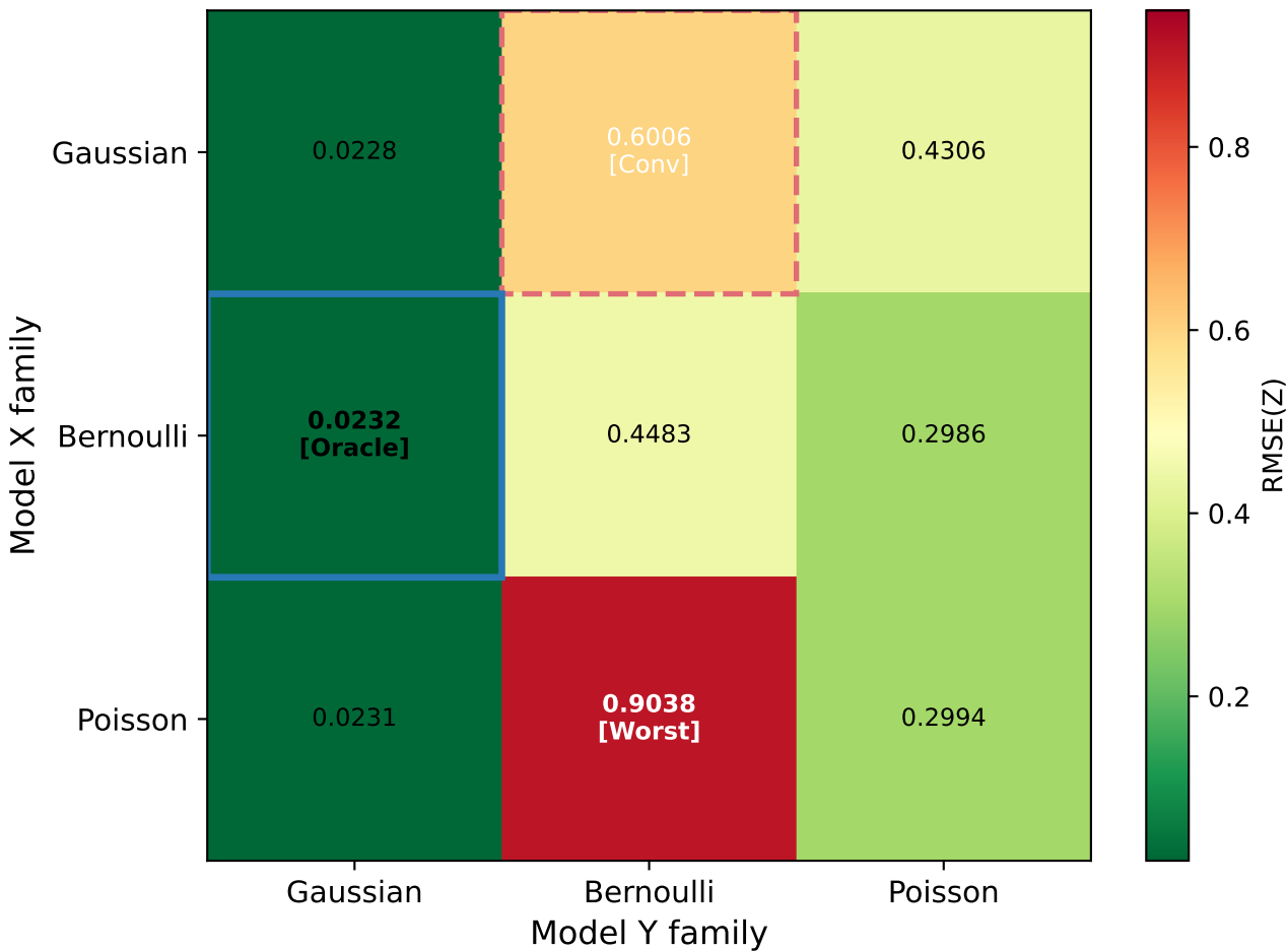
Scenario C RMSE(Z) [Fixed model: no 0.5] True: X=Bernoulli, Y=Gaussian (n=150, d=15, k=3, 10 trials)
