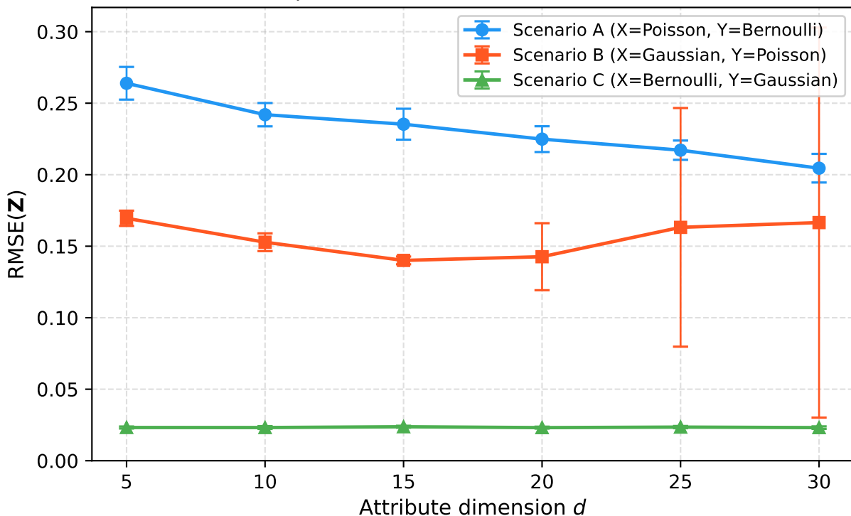
d-sweep: RMSE( \mathbf{Z} ) vs. Attribute Dimension (fixed implementation, 10 trials, n = 150 , k^* = 3 )
