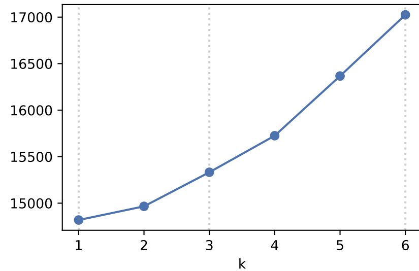
BIC vs k
