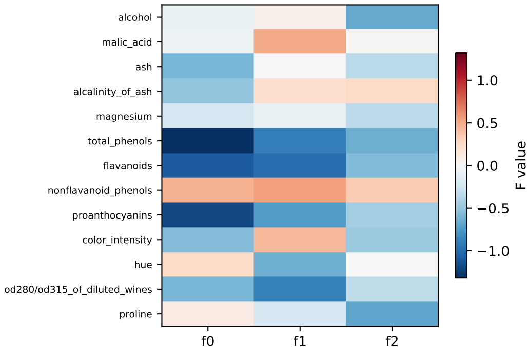
wine F heatmap (k=3, best trial=1, BIC=6353.2)
