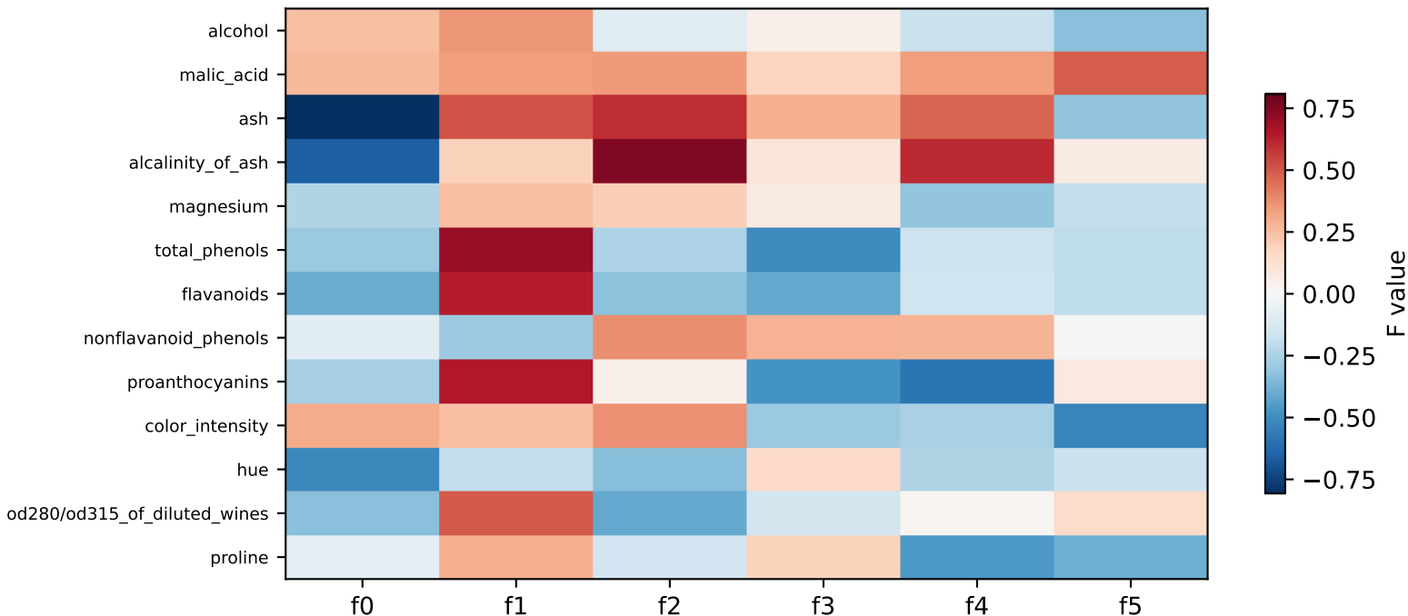
wine F heatmap (k=6, best trial=1, BIC=7444.2)
