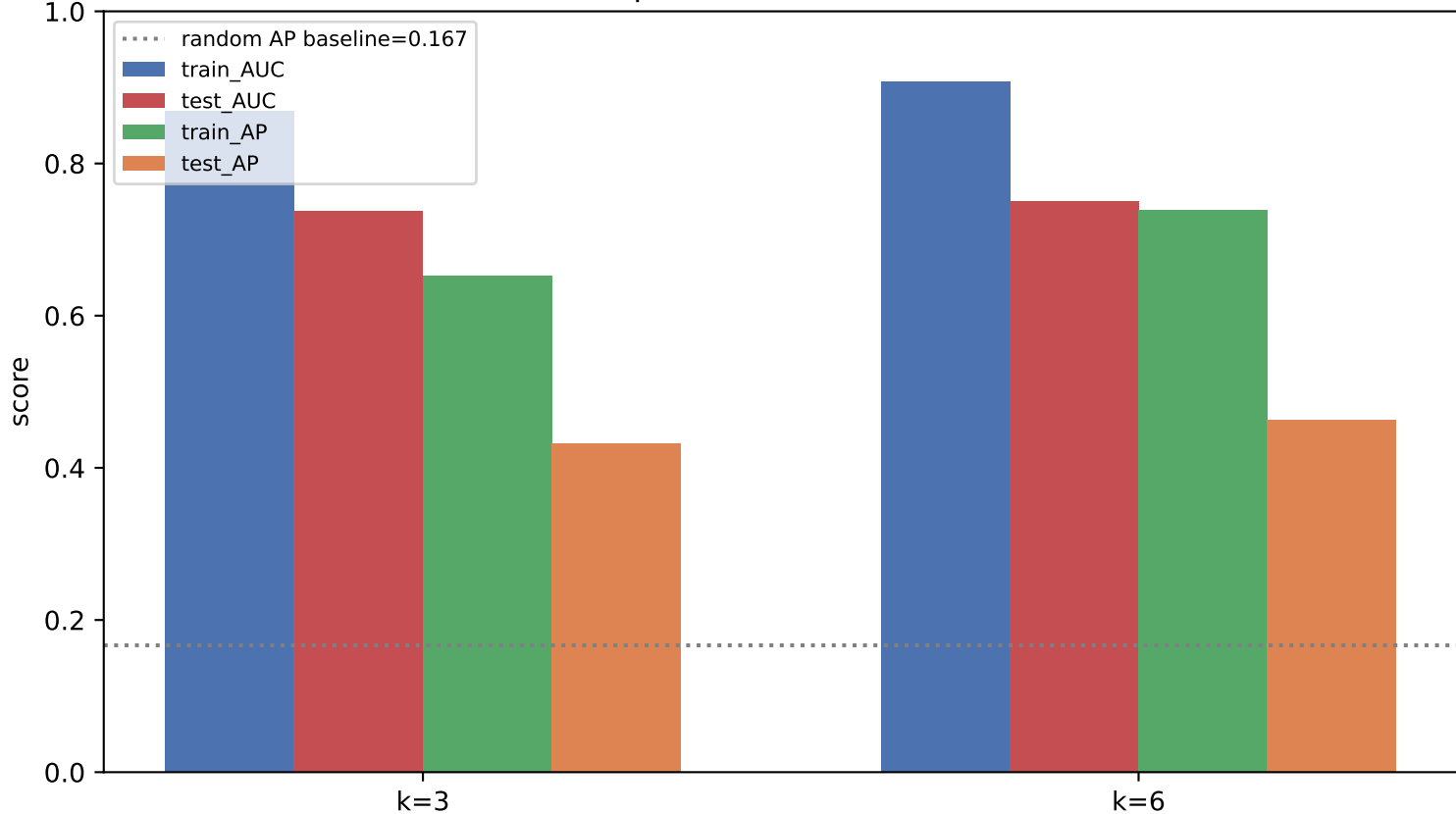
Cora held-out link prediction: train vs test (k=3 vs k=6)
