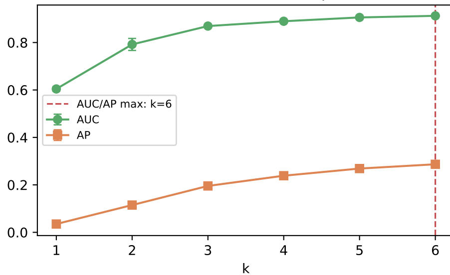
Link reconstruction (in-sample) vs k
