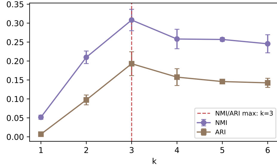
Label structure vs k
