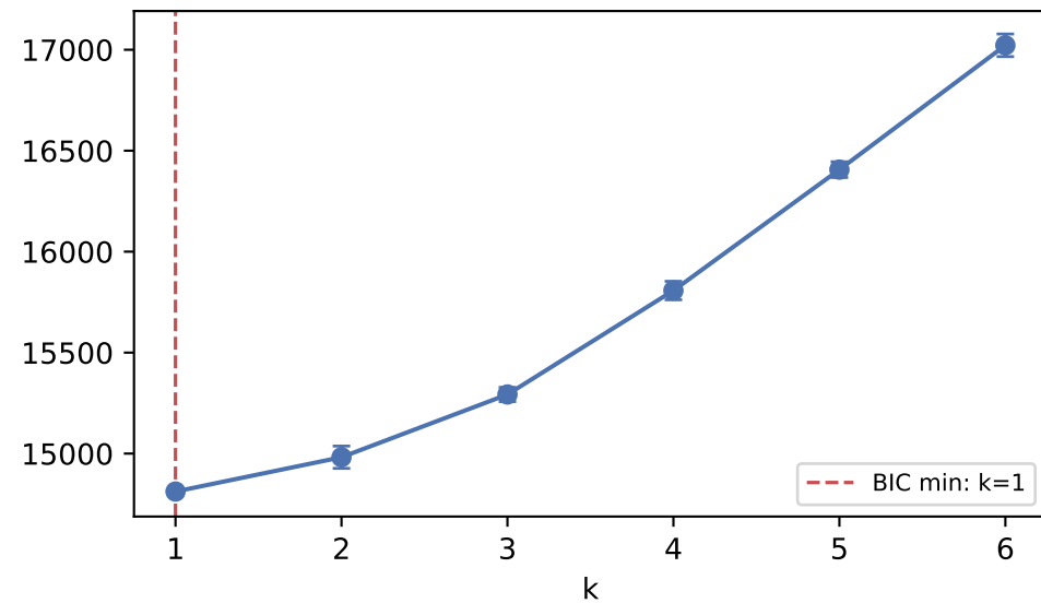
BIC vs k
