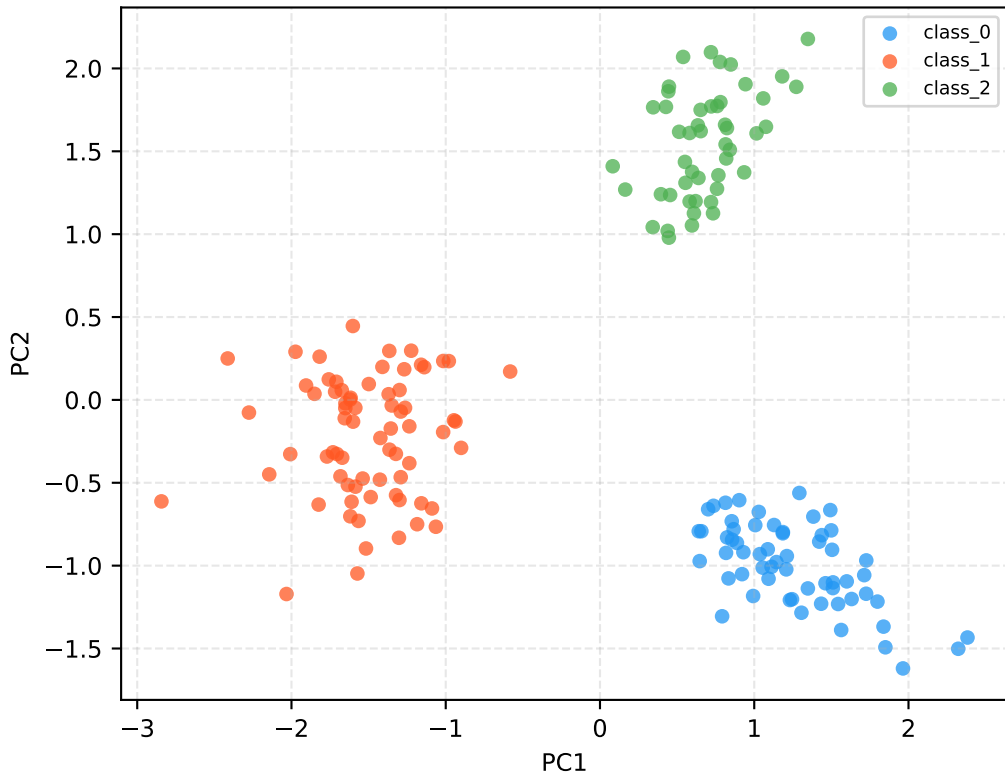
Wine Pilot: Z visualization (X+Y, k=3, PCA 2D)
